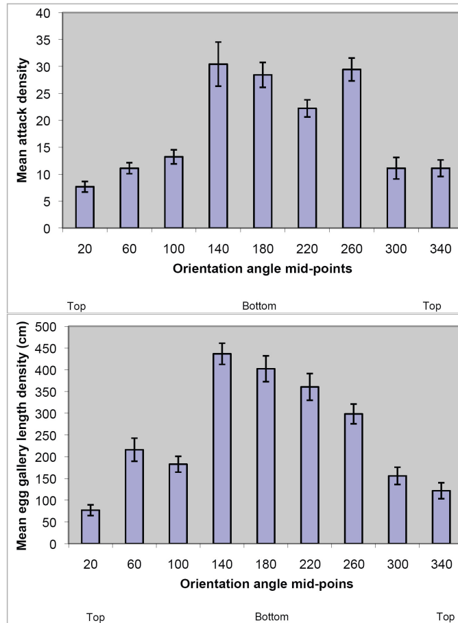
Figure 3. Empirical circular distribution of mean attack density/m 2 ( \pm 1 SE) and egg gallery length/m 2 ( \pm 1 SE) by the spruce beetle on spruce windthrow oriented north-south.
